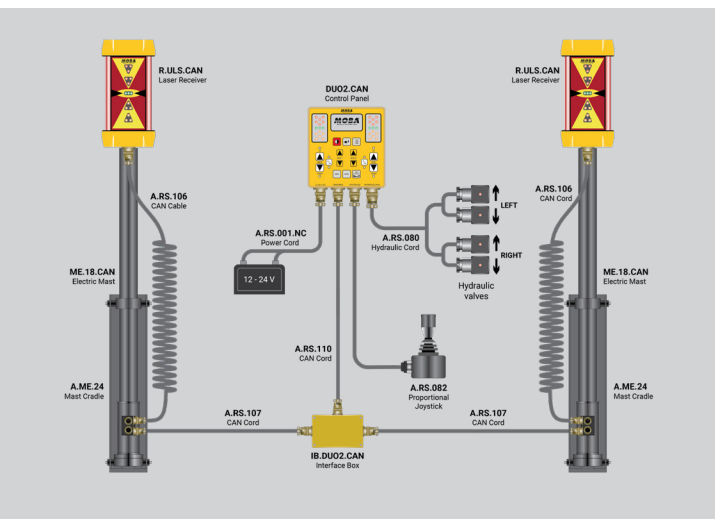
RS.037 Typical dual receiving system
