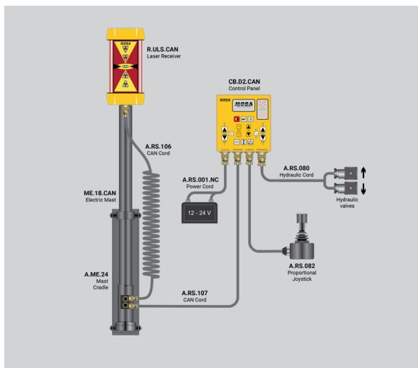
RS.033 Typical single receiving system
